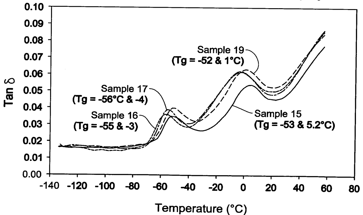
Fig. 4 Tan \delta of Plasticized Propylene Impact Copolymers
